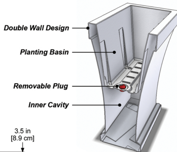
Sectional View
